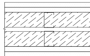
STC - 64 Chase Wall Balanced - (TL 17-292)
