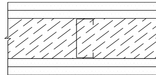
STC - 55 Single Wall Balanced - (TL 17-288)
