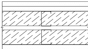
STC - 63 Chase Wall Unbalanced - (TL 17-293)
