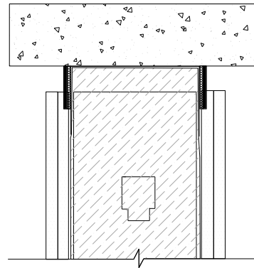
STC - 55 Single Wall Balanced - (TL 17-288)
