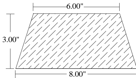
2" Deck DPW-368
