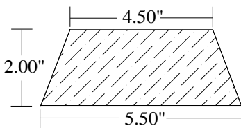
1 1/2" Deck DPW-24555
