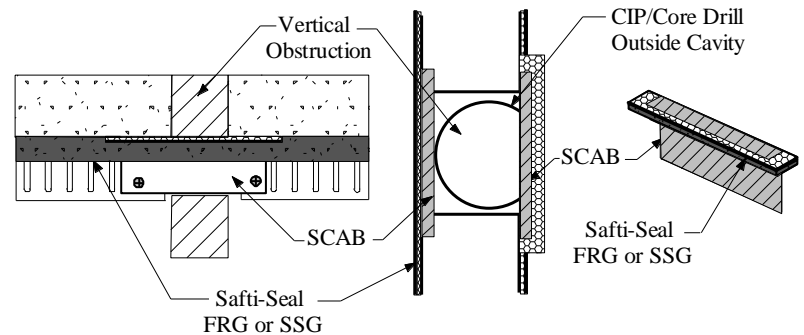
Obstruction Outside Cavity
