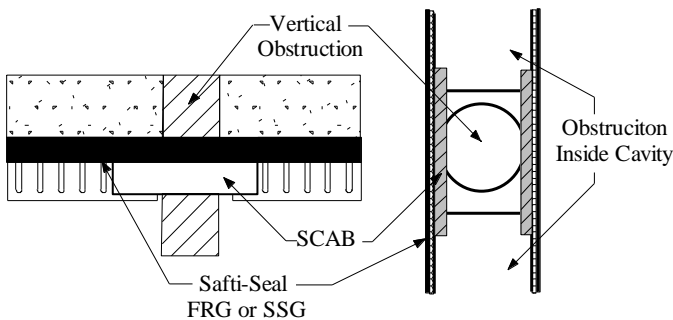
Obstruction Inside Cavity
